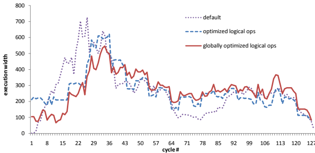
Figure 14: The 10-bit CLA program uses logical CNOT and Toffoli operations. Utilizing the optimized logical operators reduced the peak execution width from the default 726 ops to 622 ops. Globally optimizing the scheduling of these improved logical operators further reduced the peak execution width to 546 ops.
