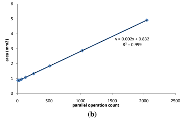
Figure 6: (a) Increasing the execution parallelism (size of instruction bundle and number of opzones in the QPU) results in linear increases in the operand transportation time. (b) The area of the QPU network increases linearly with parallelism.
