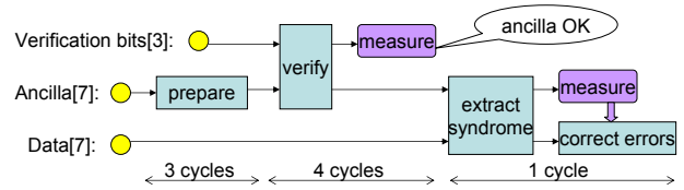
Figure 9: The simplest error recovery process: prepare the ancilla block to a specific encoded state; verify that the state is free of X errors; and extract a syndrome by interacting the ancilla with the data block. The ancilla is then measured and decoded via classical processing to determine a syndrome and the proper corrective procedure for the data block. The times listed are in terms of 2-qubit operation cycles, which are roughly 1 ms each for the eSHe QC.
