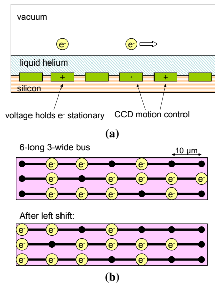
Figure 1: (a) A side view of the eSHe system (not to scale). Electron qubits float in a vacuum above a layer of liquid helium. Positively charged metal gates underneath the liquid helium attract these electrons and hold them stationary. The electrons can be moved via CCD control of these gates. (b) An example of a qubit transportation bus. Qubits move left or right along this bus akin to a shift register.
