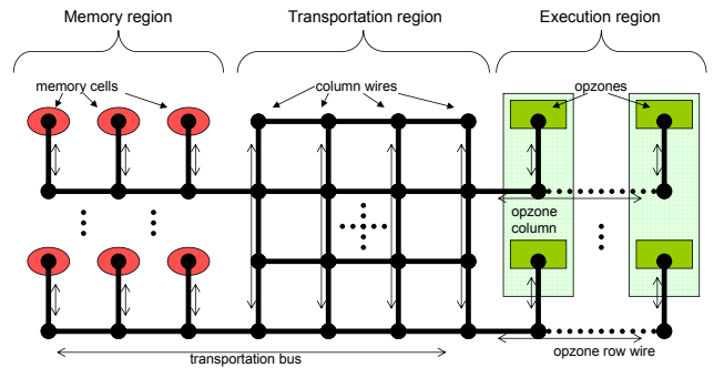
Figure 4: The Quantum Processing Unit is composed of a memory region and an execution region coupled by a transportation region. This diagram is not drawn to scale. The actual transportation region contains 9 columns, and the opzone columns are separated from each other by 100 \mu\text{m} . The double-headed arrows indicate CCD control. A single transportation bus signal controls all left-right movement in the memory and transportation regions. The memory and execution regions may be scaled by adding rows or columns to increase memory and execution capacity.
